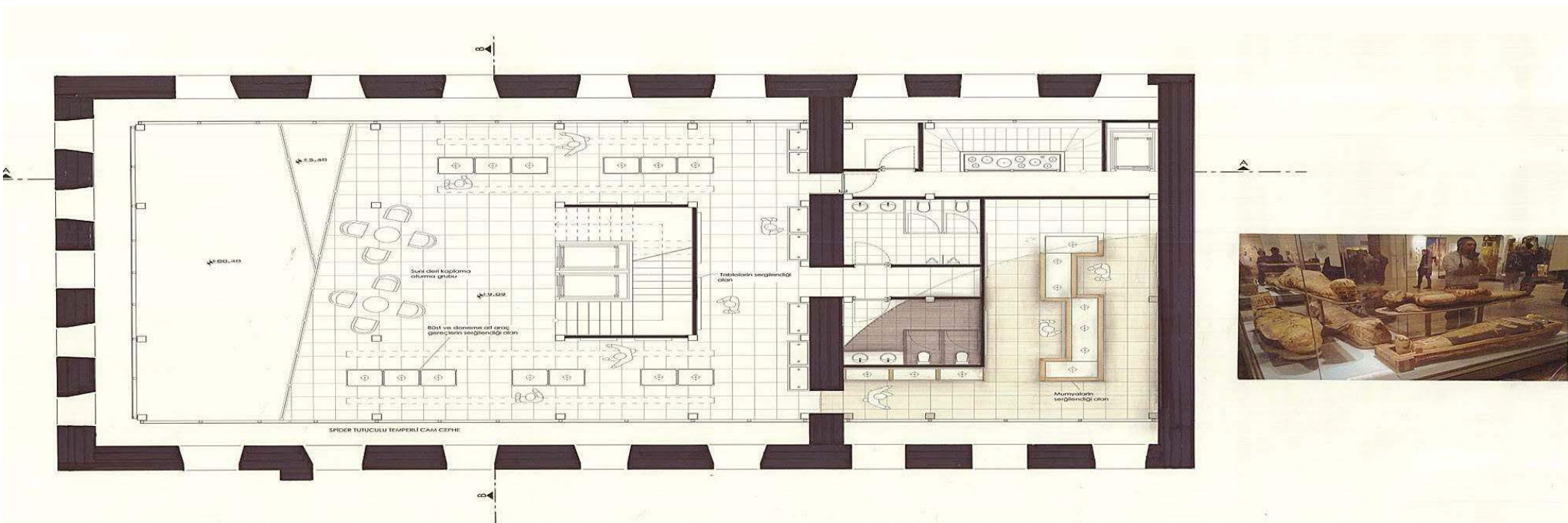
SECOND FLOOR PLAN S:1/50
